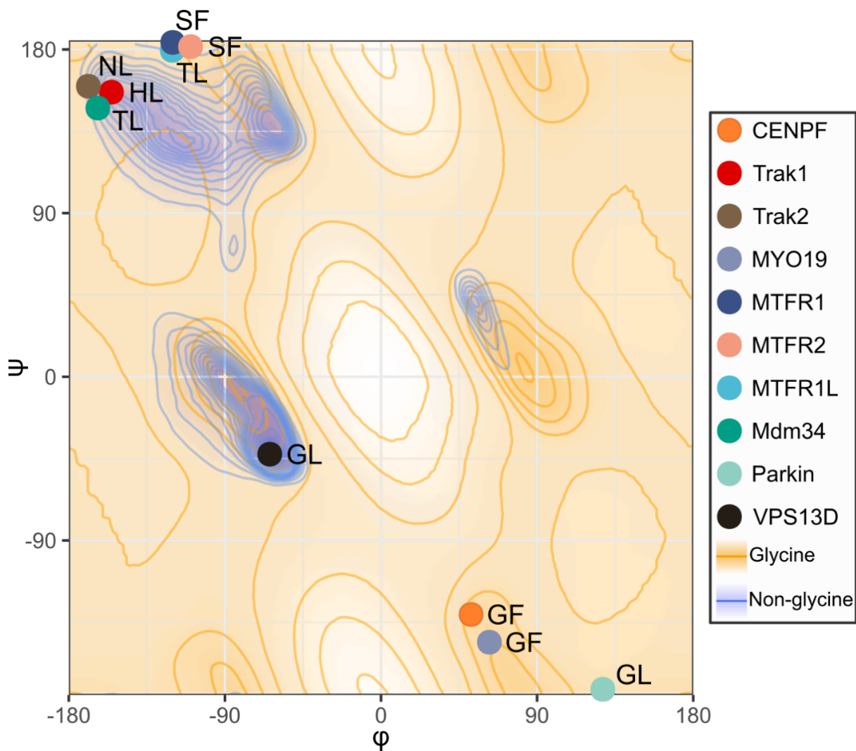
Appendix Figure S1. Angle requirements of different Miro-binding motifs. (A) Ramachandran plot depicting the bond angles of the residue preceding the ELF-binding F or L from different Miro-binding motifs. Blue and Orange depict the areas tolerating non-glycine and glycine residues respectively.
