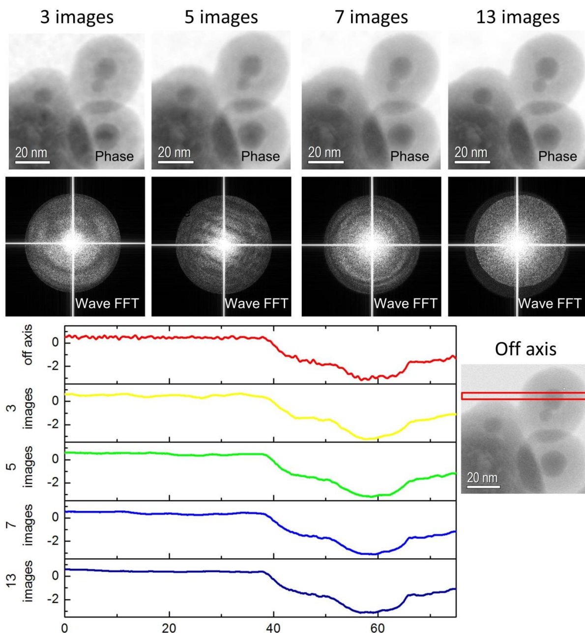
Supplementary Figure 3: Illustration of the effect of the number of defocus steps used for the reconstruction. Top row: phase images reconstructed using the different numbers of defocus images indicated. Middle row: Fourier transforms of the images in the top row. Bottom row: phase profiles obtained from the region marked in red in the off-axis phase image shown on the right.
