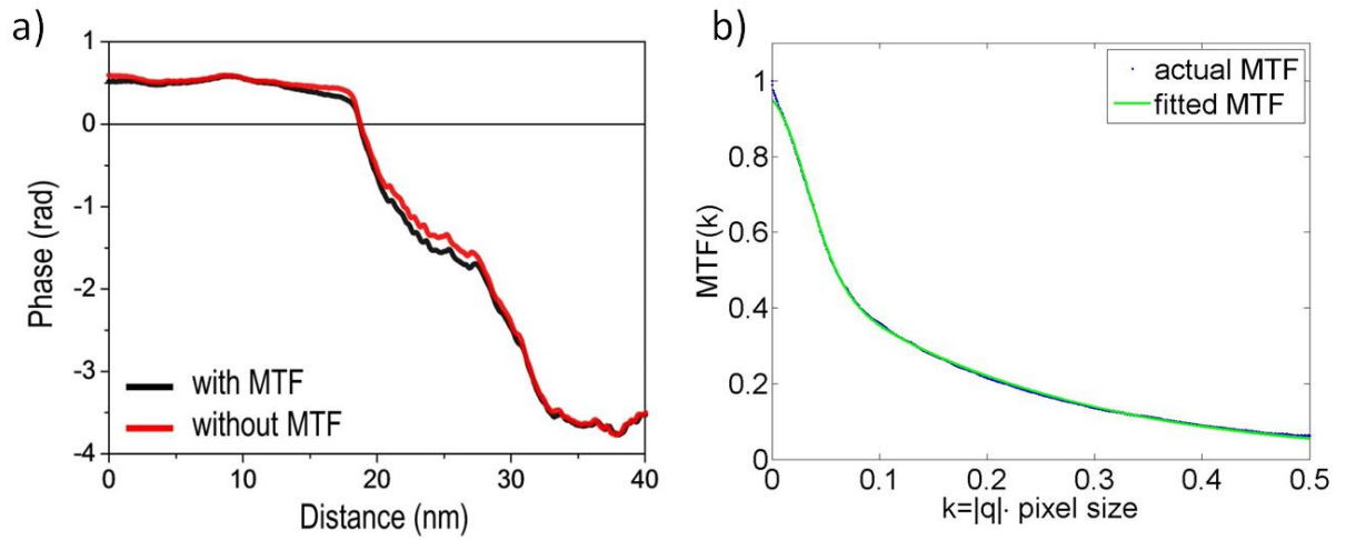
Supplementary Figure 4: The effects of MTF a) Illustration of the effect on the phase profile of taking the MTF of the CCD camera into account. b) MTF of the CCD camera being used for this experiment. In order to smoothen the MTF for use in the reconstruction the following equation was fitted to it: \text{MTF}(k) = 0.5559 \cdot \exp(-4.6362 \cdot k) + 0.3925 \cdot \exp(-458.2232 \cdot k^2) [3]. The abscissa and k in this expression are both the normalized spatial frequency, i.e. the spatial frequency |q| multiplied by the detector pixel size, so that k_{\text{Nyquist}} = 0.5 . The MTF data measured for the 10 lowest values of k were not included in the fit.
