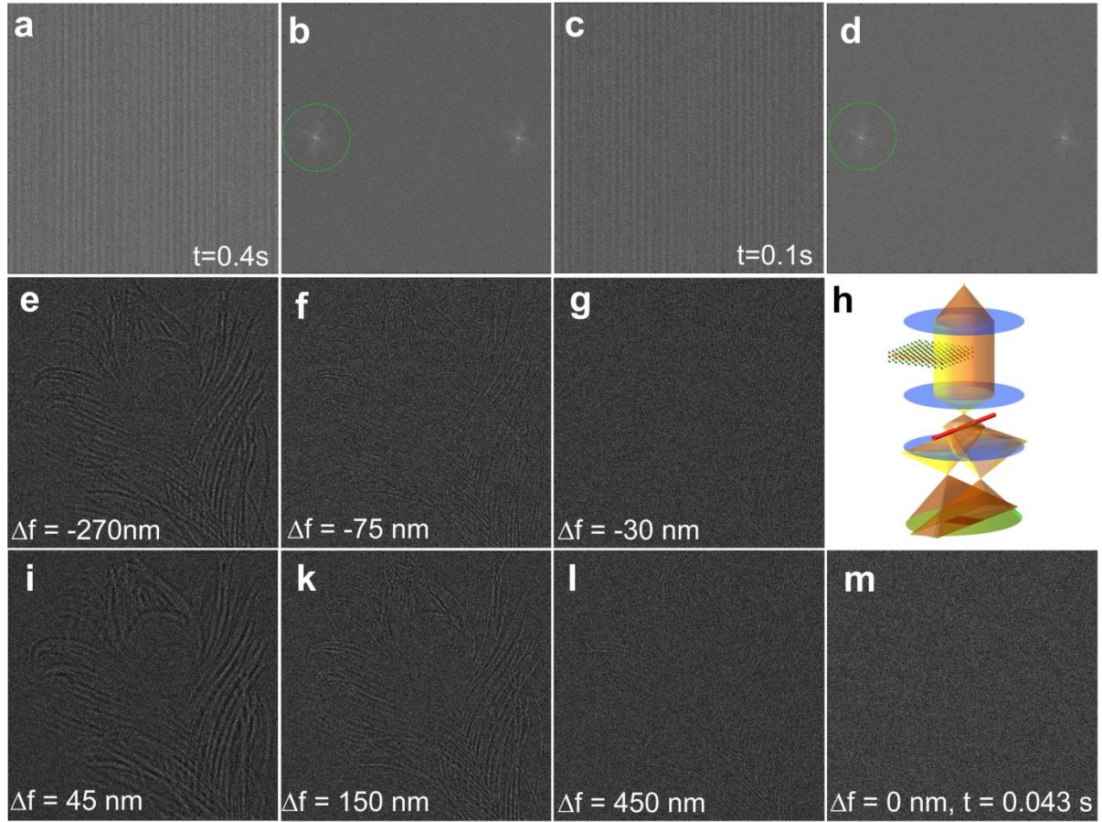
Supplementary Figure 5: The effect of exposure time: Simulated 80 kV off-axis and inline holography data used to recover the phase images shown in Fig. 4. Poisson noise has been added in order to simulate the effect of finite exposure time. Round illumination ( \varepsilon=1 ), a source brightness of \beta = 2 \cdot 10^8 \text{ Acm}^{-2}\text{sr}^{-1} , a pixel size of 0.1 nm, and a field of view of 80 nm have been assumed. (a) Off-axis hologram simulated for an exposure time of 0.4 s. The shear distance x_{\text{Shear}} was equal to the field of view, and an optimized illumination semi-convergence angle of \alpha = \lambda/(\sqrt{2} \pi x_{\text{Shear}}) = 11.7 \mu\text{rad} was assumed [4]. Fresnel fringes due to the biprism have not been simulated. (b) Fourier transform of (a). (c) and (d) Off-axis hologram and FFT for an exposure time of 0.1 s. The green circles in (b) and (d) indicate the size and position of the numerical aperture used to reconstruct the wavefunction. (e), (f), (g), (i), (k), (l), and (m) show the inline holograms simulated for the indicated planes of focus and exposure times of 0.043 s, adding up to a total of 0.3 s for the complete series. The illumination conditions were chosen identical to those used for the off-axis simulation. (h) Round illumination ( \varepsilon=1 ) and a high spatial coherence (the small \alpha specified above) were assumed, in agreement with the experiment.
