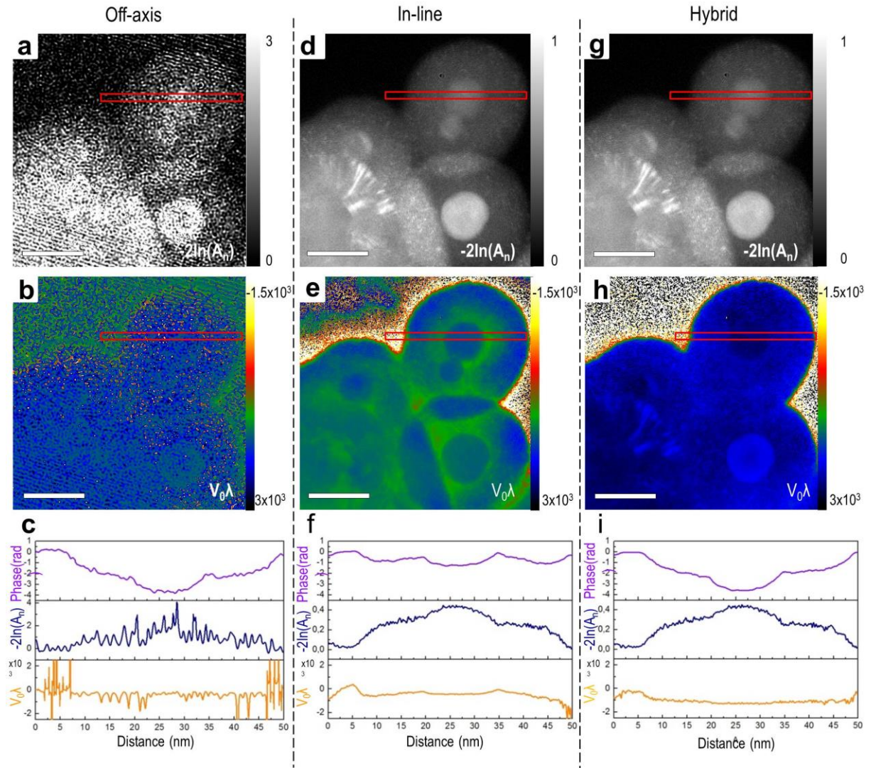
Supplementary Figure 2: Thickness independent inner potential maps: Top row (a,d,g): The inverted logarithm of the reconstructed amplitudes (specifically -2\ln(A_n) ) calculated for the off-axis, in-line and hybrid methods. Middle row (b,e,h): thickness-independent V_0\lambda^{1,2} images calculated for the off-axis, in-line and hybrid methods. Profiles extracted from the boxes marked in red are shown in (c), (f) and (i). Scale bar, 20 nm.
