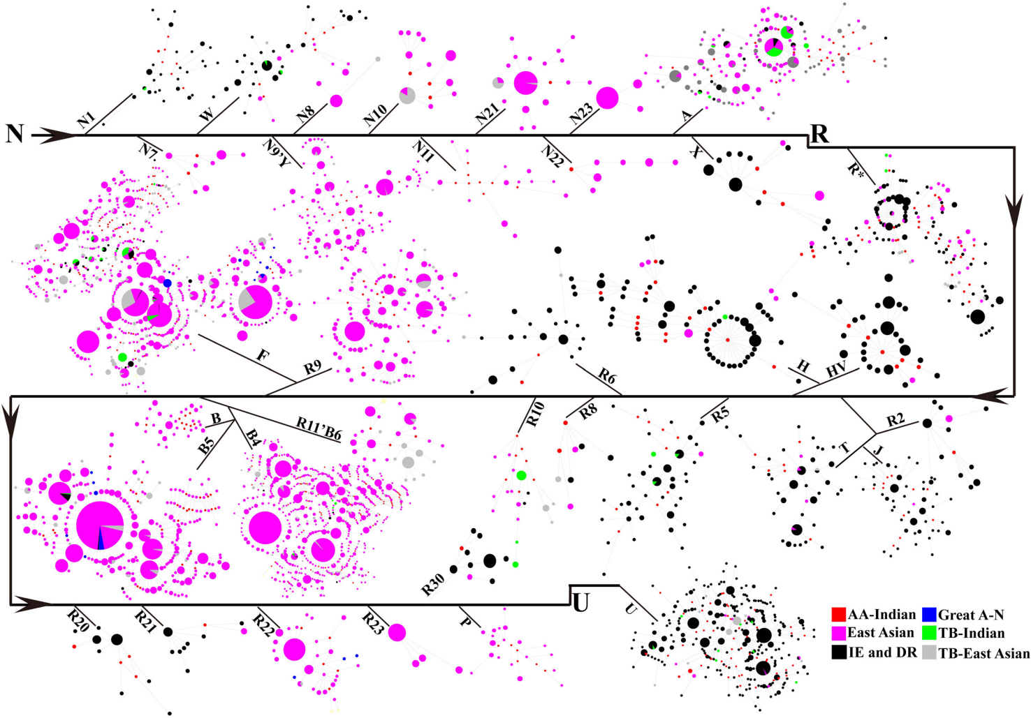
Figure S2. Network of mtDNA lineages under the macro-haplogroup N in East Asia and South Asia populations. The mtDNA data is collected from the references in supplementary Table S7.
