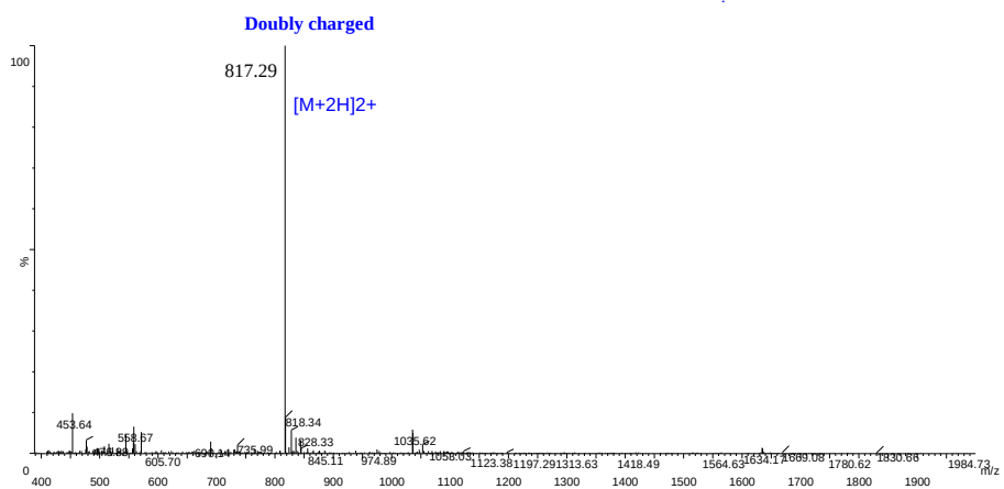
Fig2. S1. Mass spectra of [DLys 6 ]-LHRH-MTX
