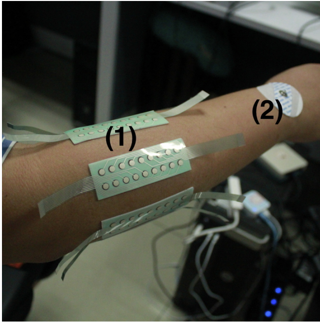
Figure S1: The MCI system: (1) electrode array; (2) reference electrode; (3) acquisition modules; (4) data transmission module; (5) lithium battery; (6) instantaneous sEMG image; (7) recognized gesture.
