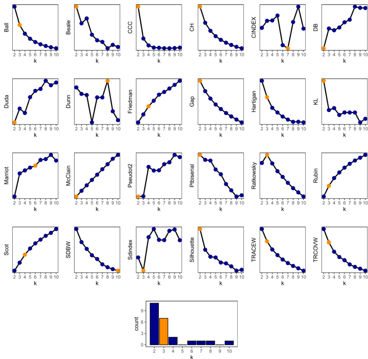
Fig.S1. Selection of the number of clusters to consider.
