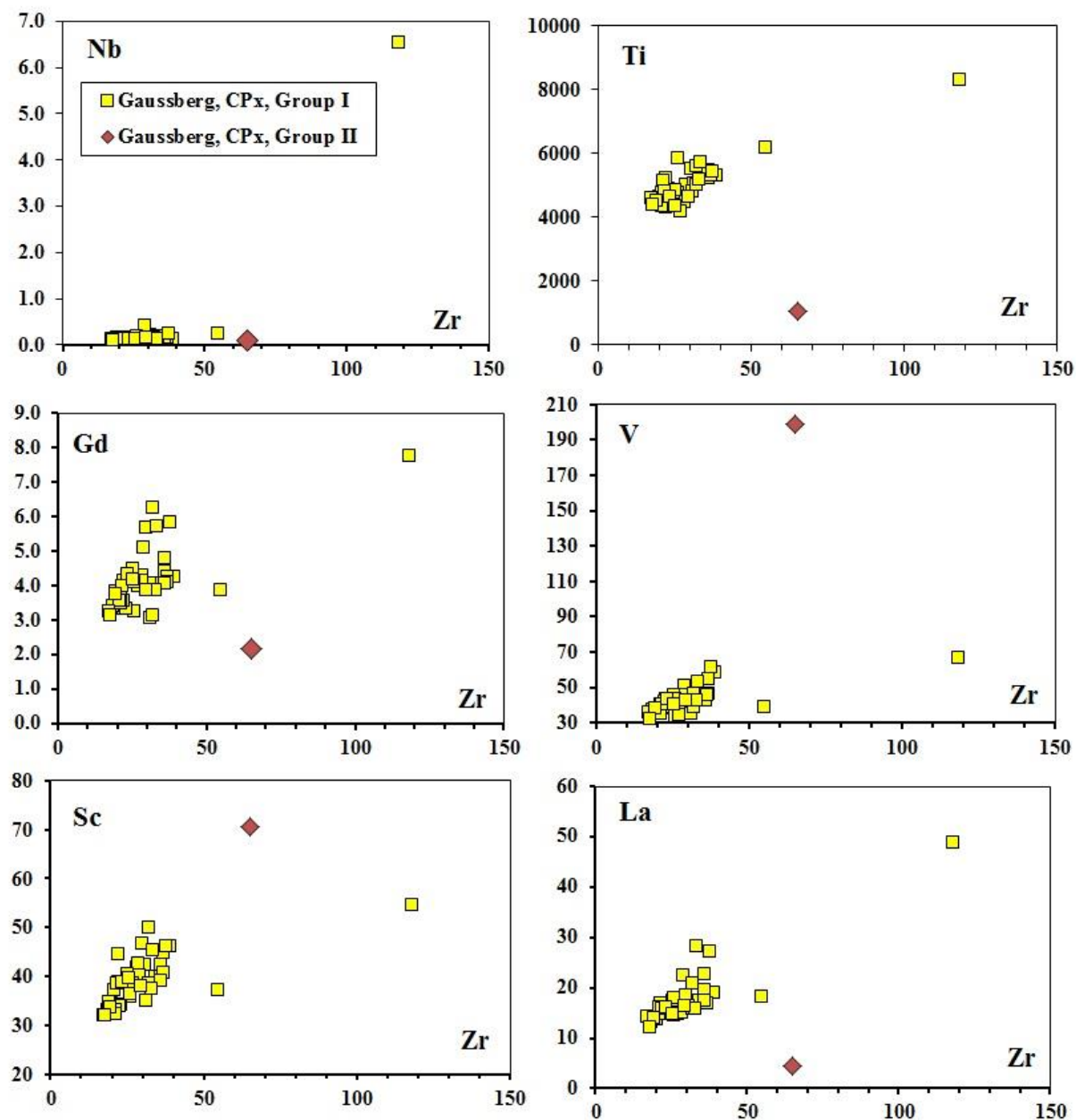
Fig. 3-S. Variations of lithophile elements (in ppm) in two groups of clinopyroxene phenocrysts from Gaussberg lamproites.
