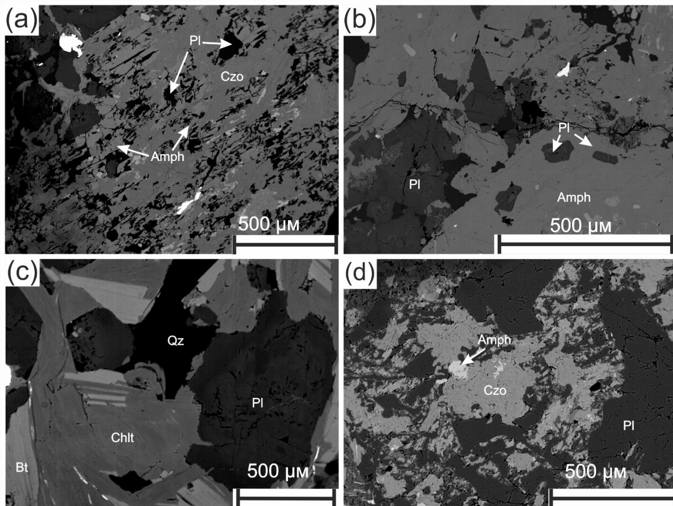
Fig. ESM 8. The relationship of minerals and structural and textural features of the dioritoids of the Podgornensky area. a – BSE image of a fragment of hornblende grain, which develops clinoclase(?) and albite(?), A3-9-19; b – BSE image of amphiboles and plagioclase grains, A3-9-19; c – contrasting BSE image of biotite replacement with chlorite, A3-22; d – BSE image of plagioclase grain, which is replaced by clinoclase, A3-22.
