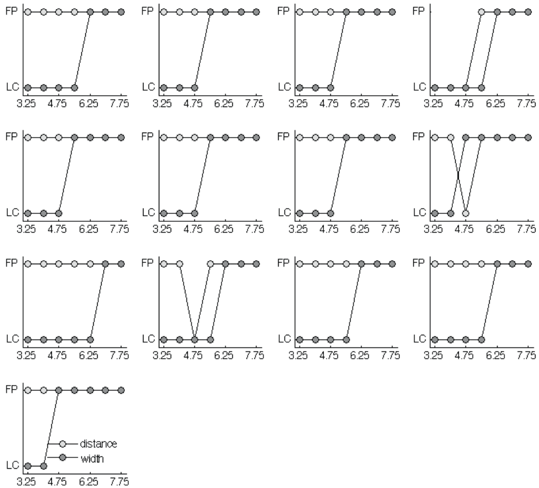
Figure: Identified attractor structures in the cyclic task for the width and distance conditions. White dots represent distance conditions; gray dots represent width conditions (legend in the lower panel only). The horizontal axis displays ID , the vertical axis sets fixed point trials ("FP") and limit cycle trials ("LC") apart. Each panel contains the data of one participant.
