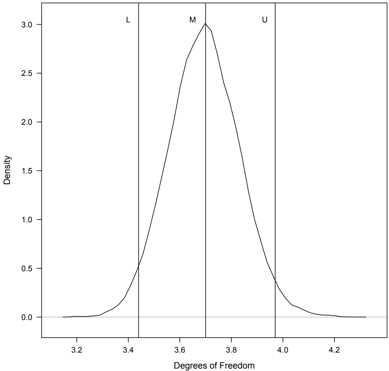
Student's t Distribution
