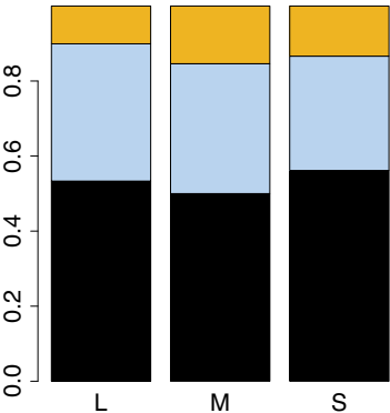
100 QTL, h^2=0.4
