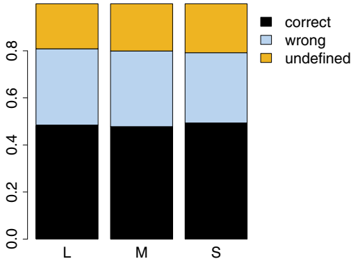
100 QTL, h^2=0.7
