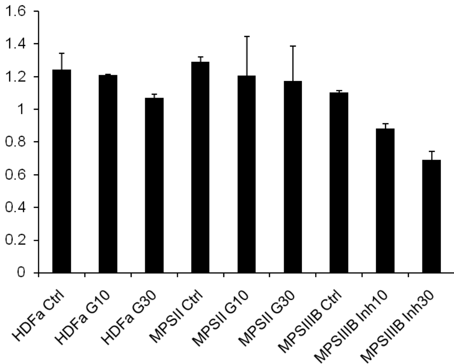
Phosphorylation of EGFR (Normalized by Total)
