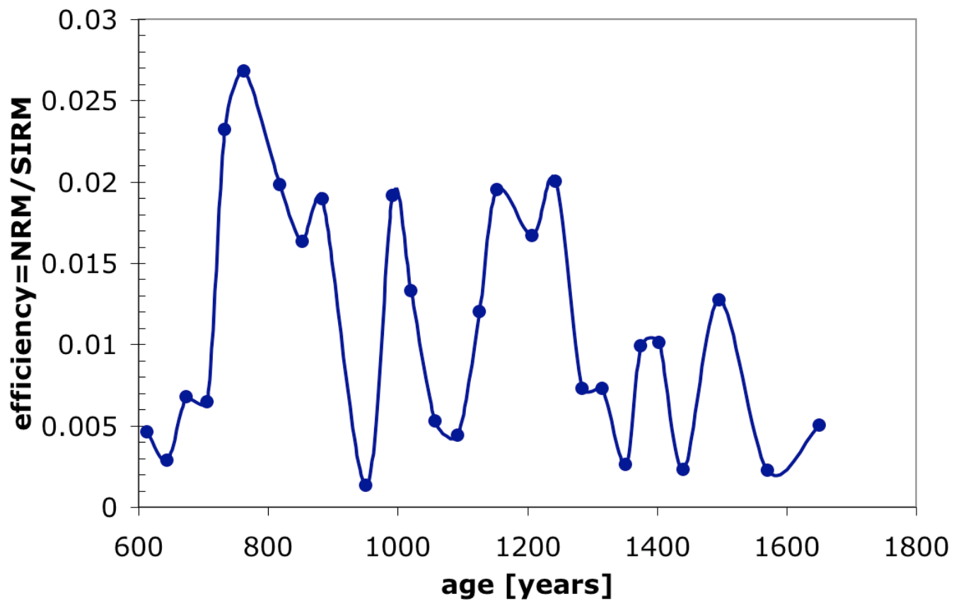
Figure 7: Efficiency of magnetization is plotted as a function of age for several samples of Sequoia sempervirens
