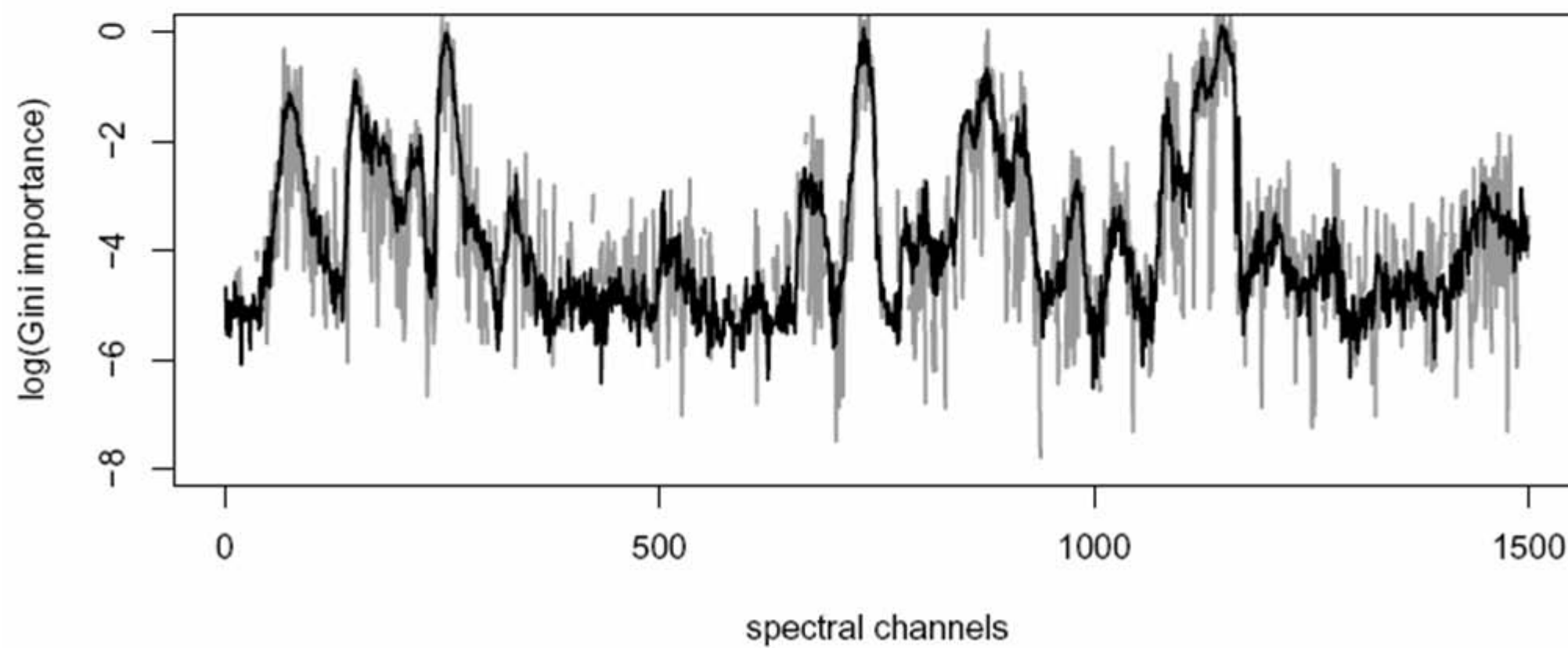
multivariate Gini importance
