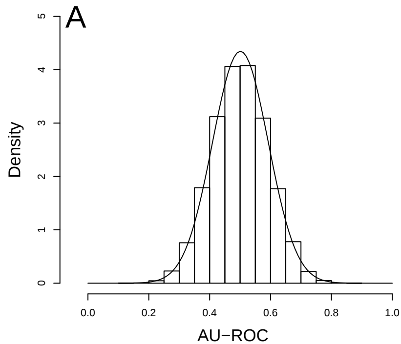
Null Distribution of BEDROC
