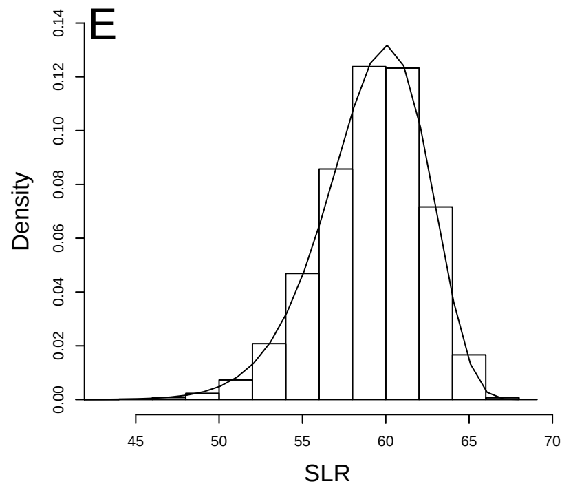
Null Distribution of SLR
