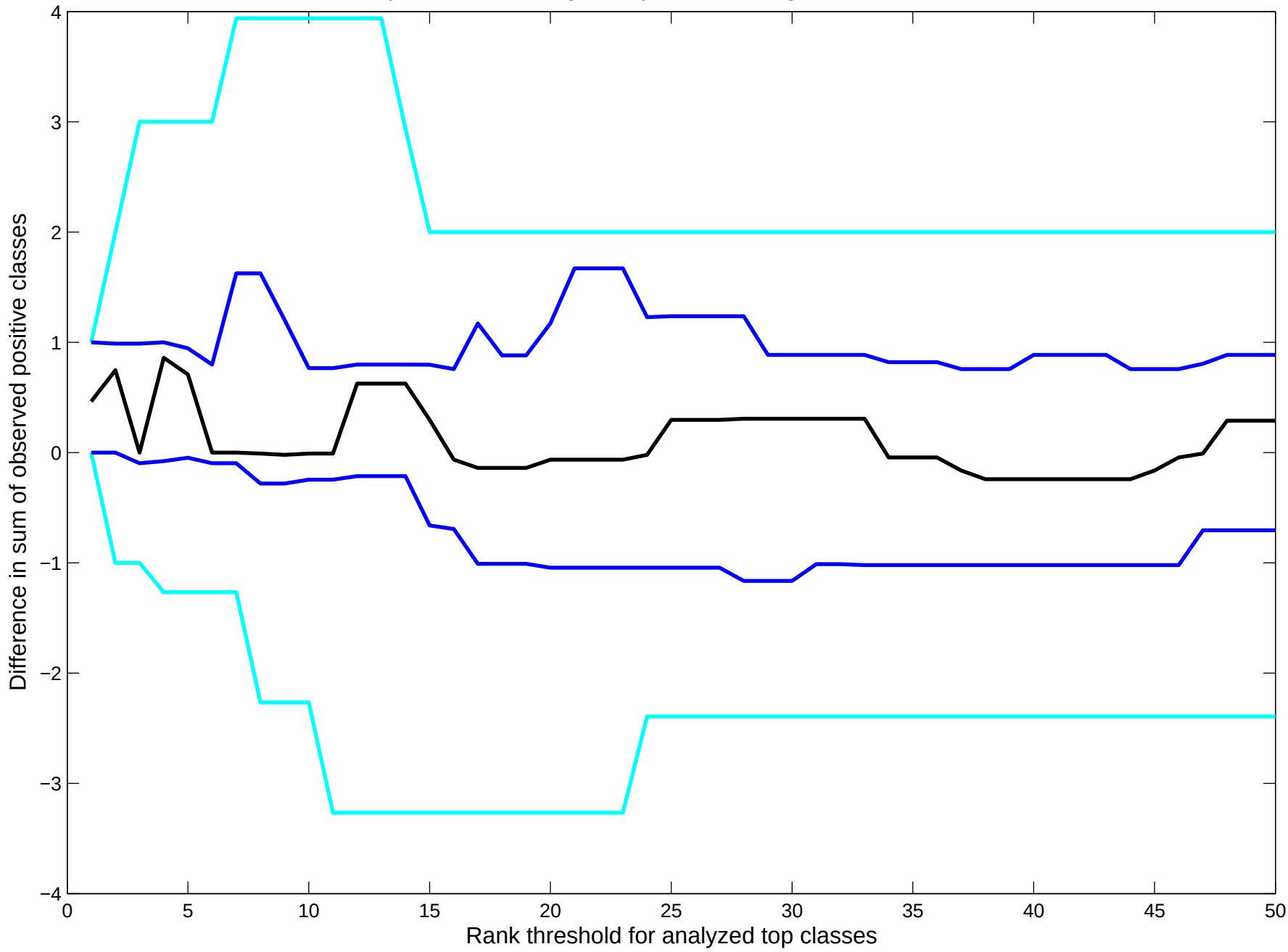
Comparison of Ontologizer top-eliminate alg. and normal GO list
