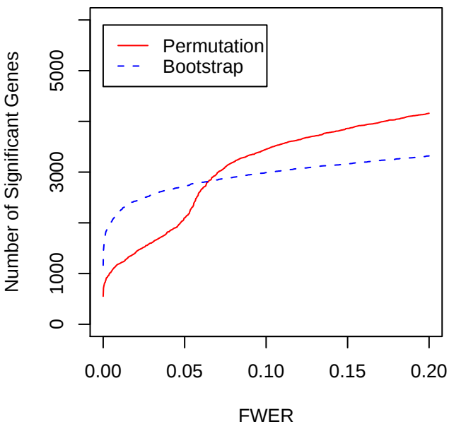
Time-Course Hypothesis
