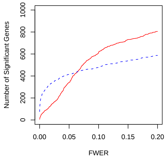
Time-Trend Hypothesis
