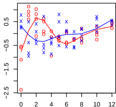
C30H6.2
