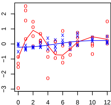
R11G11.2
