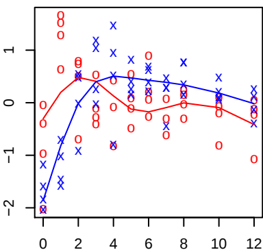
C35A11.4#2
