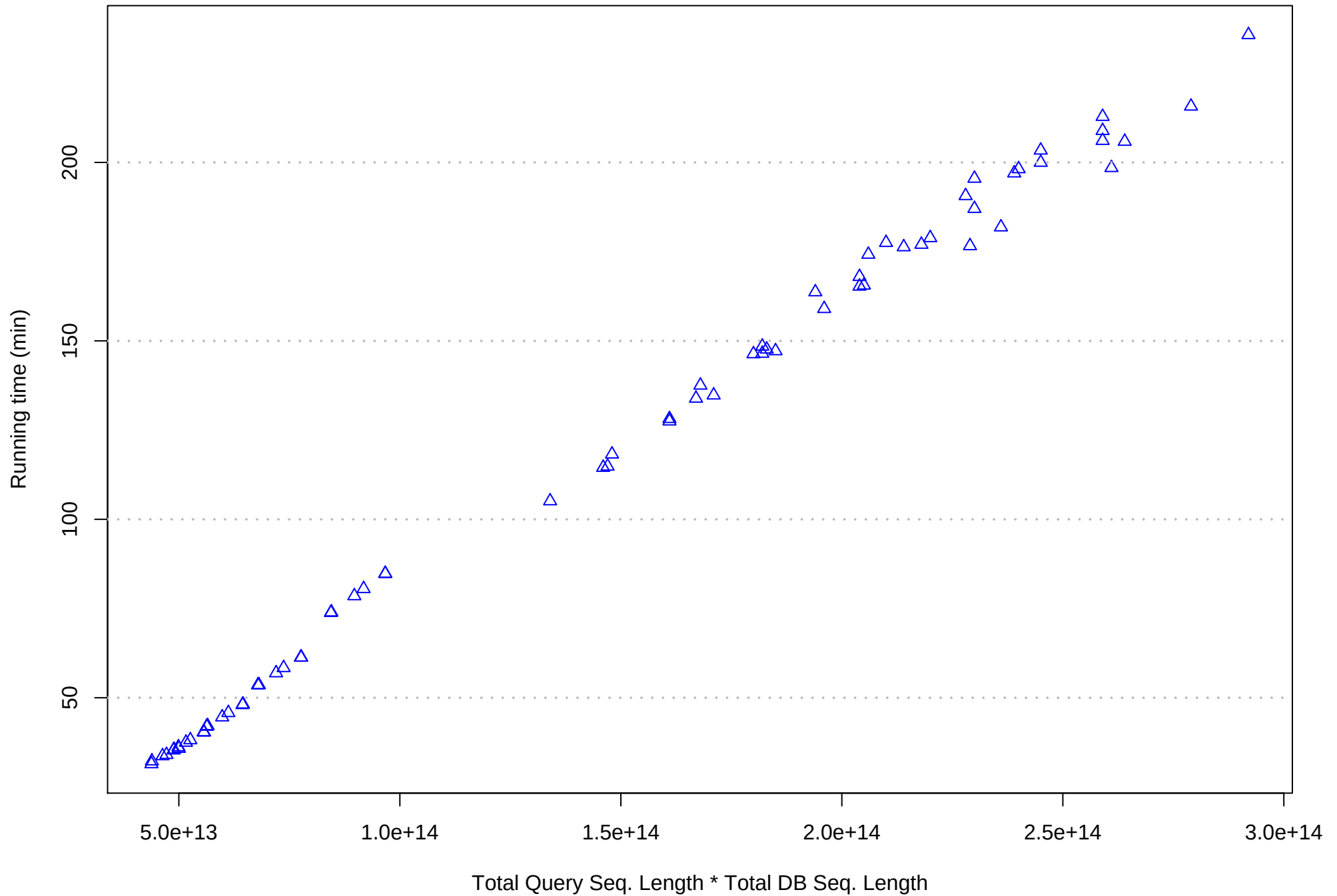
Run time with respect to search space
