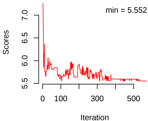
Minimum Path
