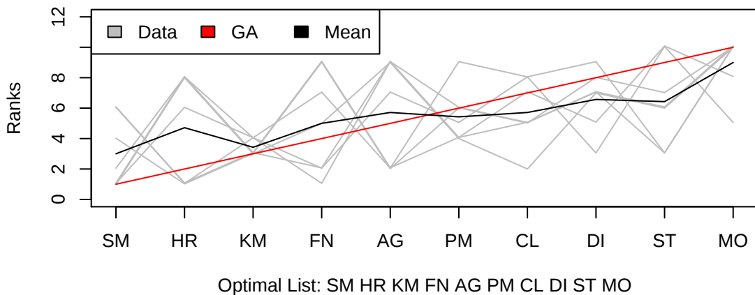
Rank Aggregation
