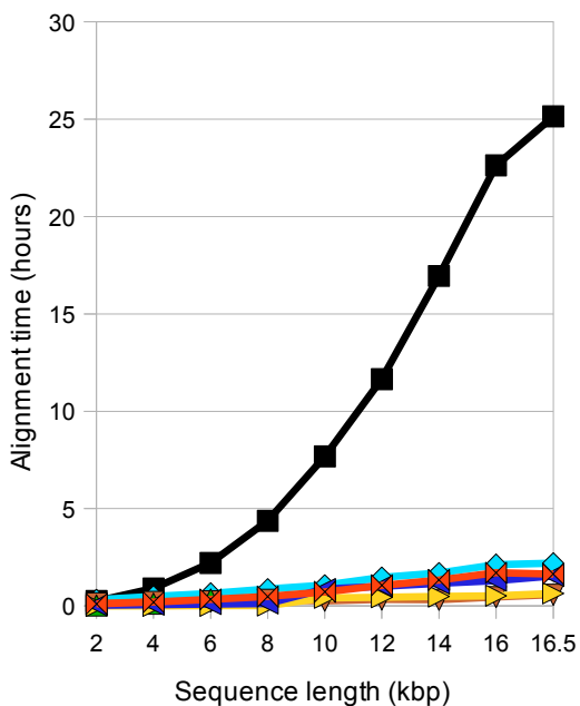
D. Human mtDNA, 400 sequences
