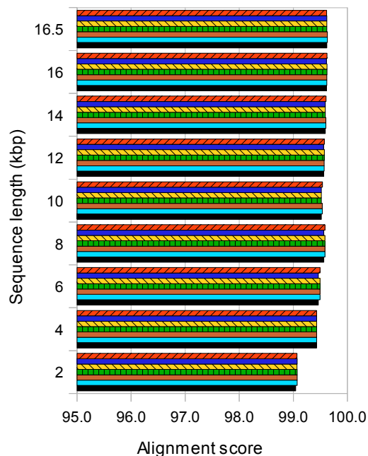
C. Human mtDNA, 200 sequences
