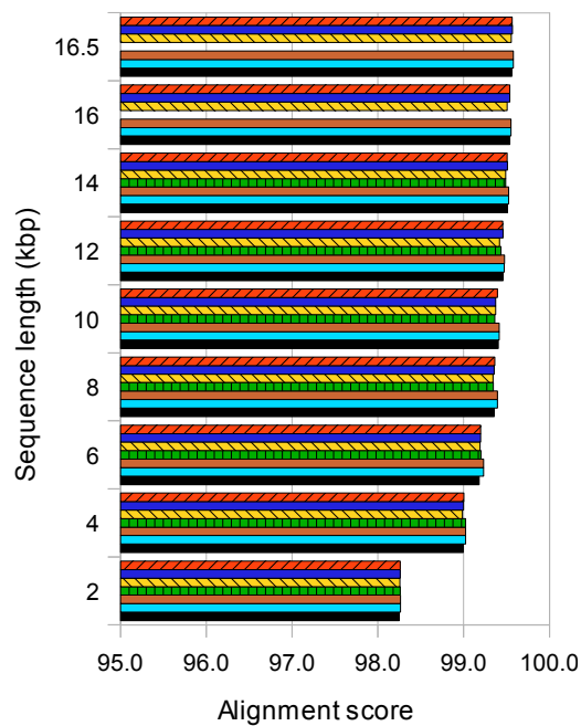
C. Human mtDNA, 200 sequences
