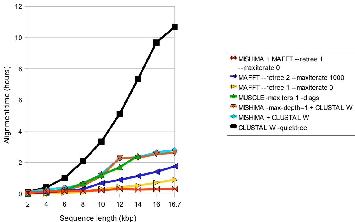
C. Mammalian mtDNA, 200 sequences
