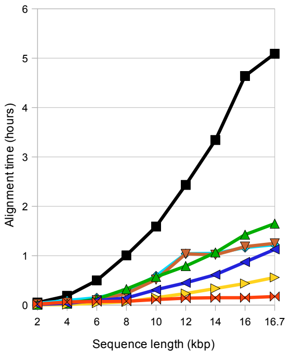
B. Mammalian mtDNA, 100 sequences
