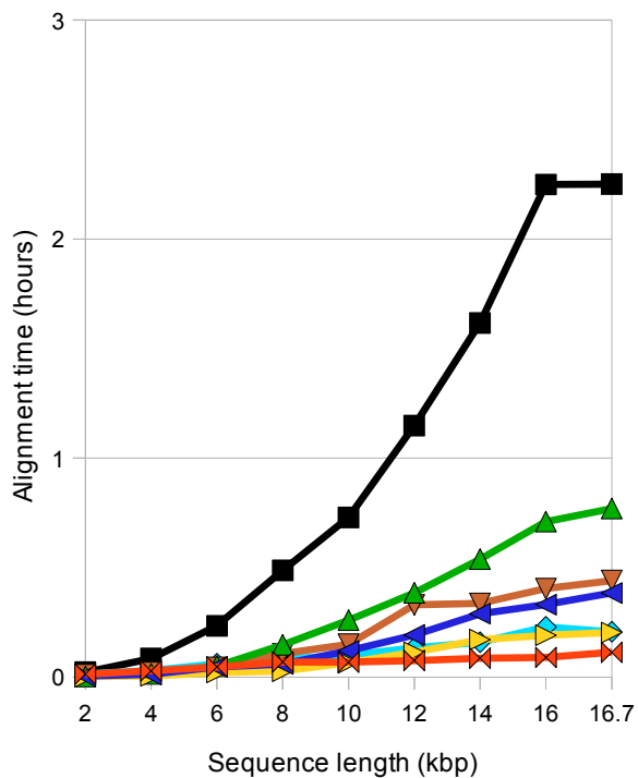
C. Mammalian mtDNA, 200 sequences
