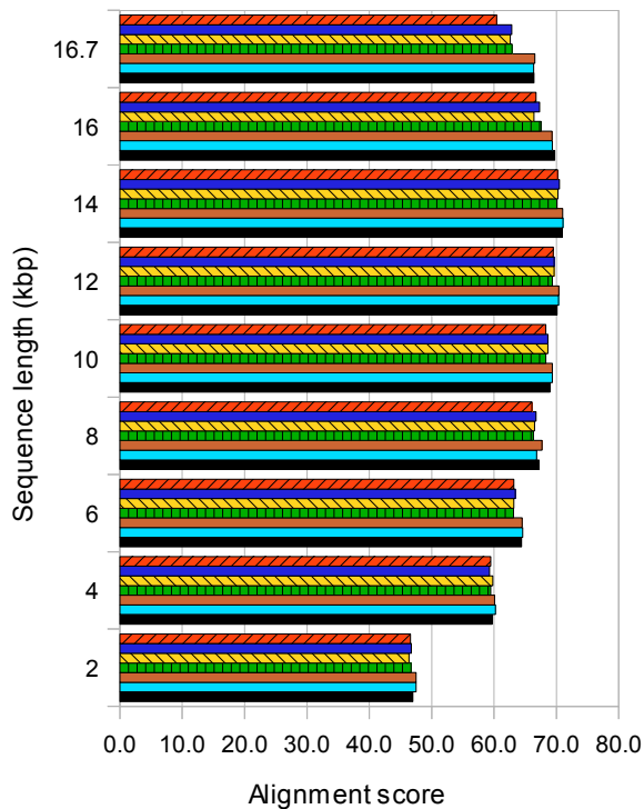
C. Mammalian mtDNA, 200 sequences
