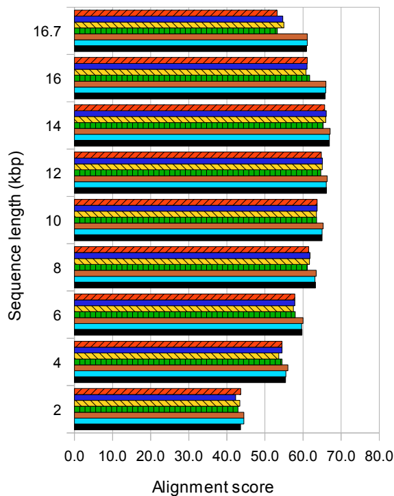
B. Mammalian mtDNA, 100 sequences
