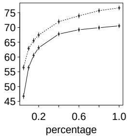
(b) Sensitivity
