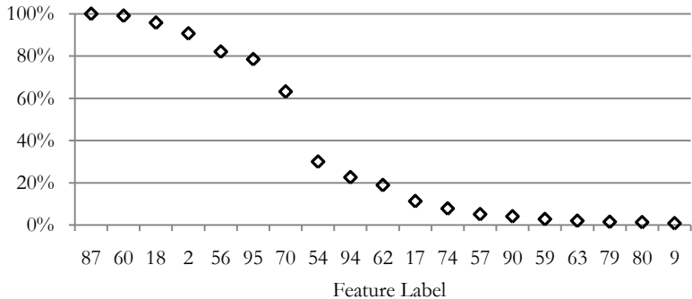
Selection Rate
