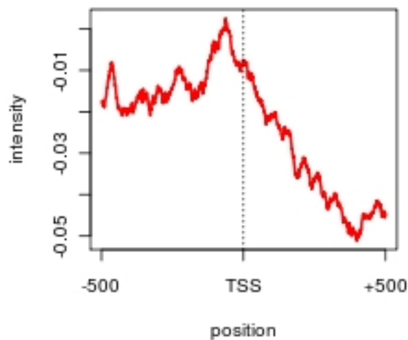
cluster 1, size=241
