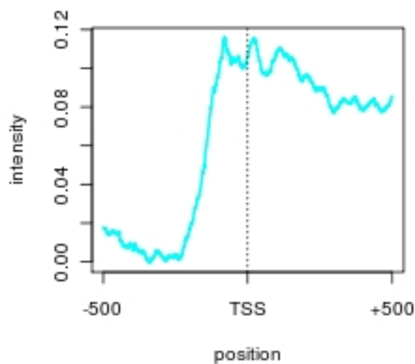
cluster 2, size=294
