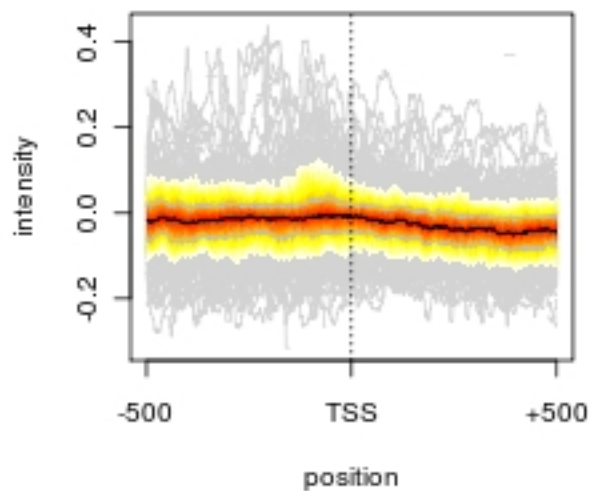
cluster 1
