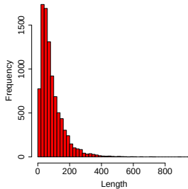
Combined Sub-HMMs
