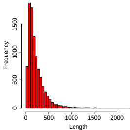
Pfam HMMs
