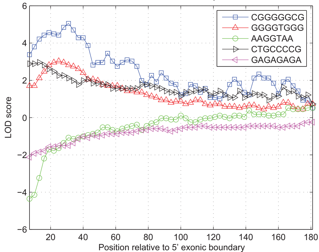
5'SS ISEs/ISSs filtered LOD profiles
