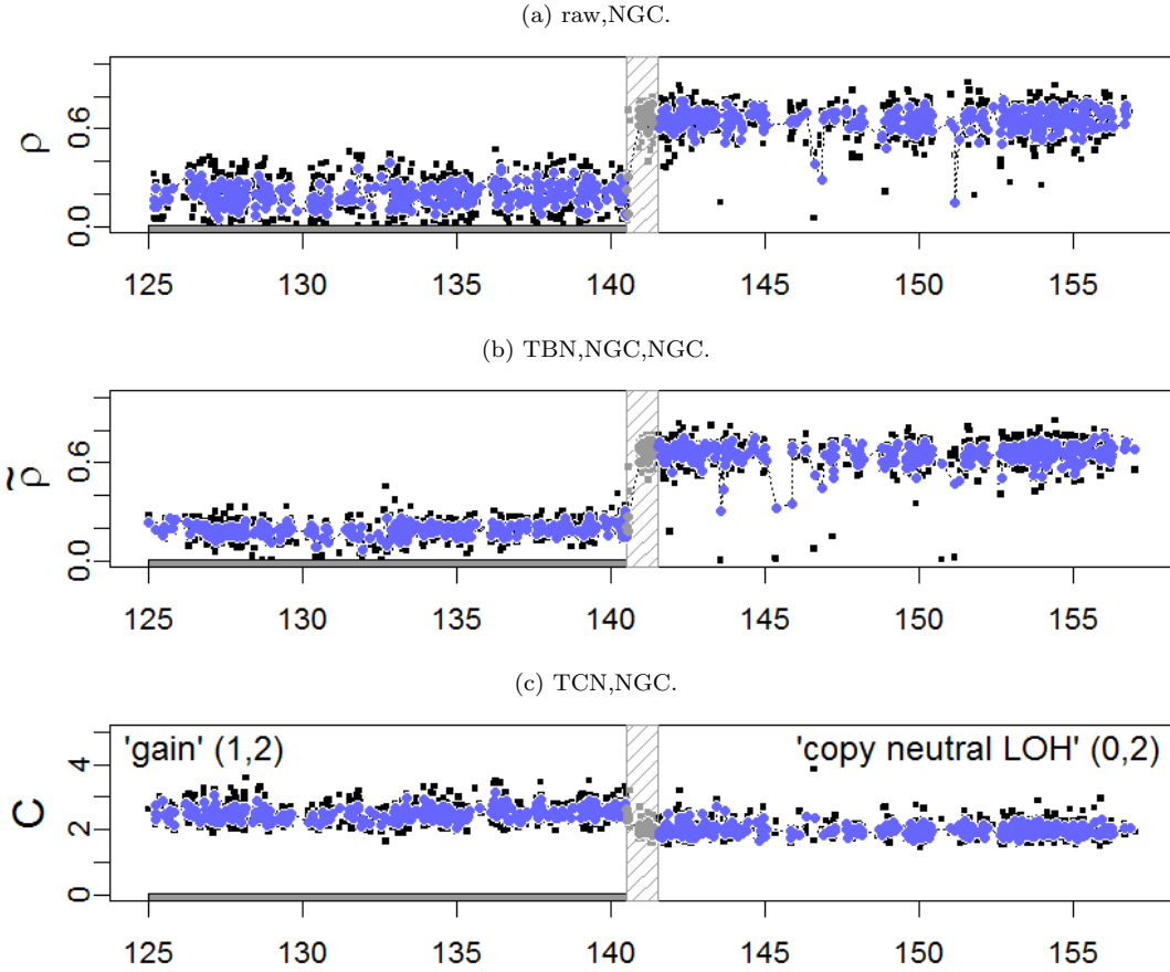
Figure 8: Decrease in Heterozygosity (DH) and total copy numbers for region TCGA-23-1027:Chr2@125.0-157.0,cp=141.0+/-0.5,s=1/3. Only heterozygous SNPs are plotted. There are 1283 loci of state 'gain' (1,2) ("negatives") and 1283 loci of state 'copy neutral LOH' (0,2) ("positives"), where the latter are highlighted with a solid bar beneath. In total 87 loci within the safety margin were excluded.
