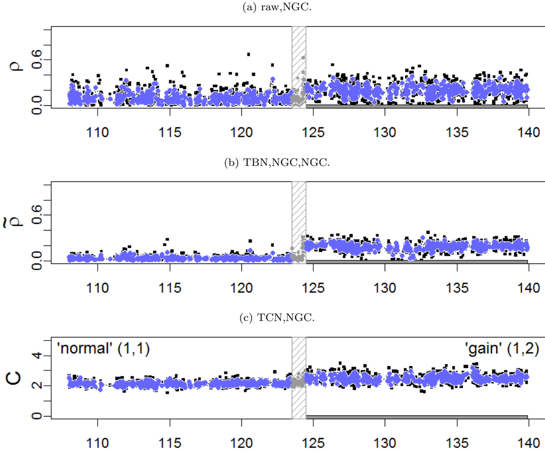
Figure 1: Decrease in Heterozygosity (DH) and total copy numbers for region TCGA-23-1027:Chr2@108-140,cp=124+/-0.5,s=0/1. Only heterozygous SNPs are plotted. There are 1634 loci of state 'normal' (1,1) ("negatives") and 1634 loci of state 'gain' (1,2) ("positives"), where the latter are highlighted with a solid bar beneath. In total 89 loci within the safety margin were excluded.
