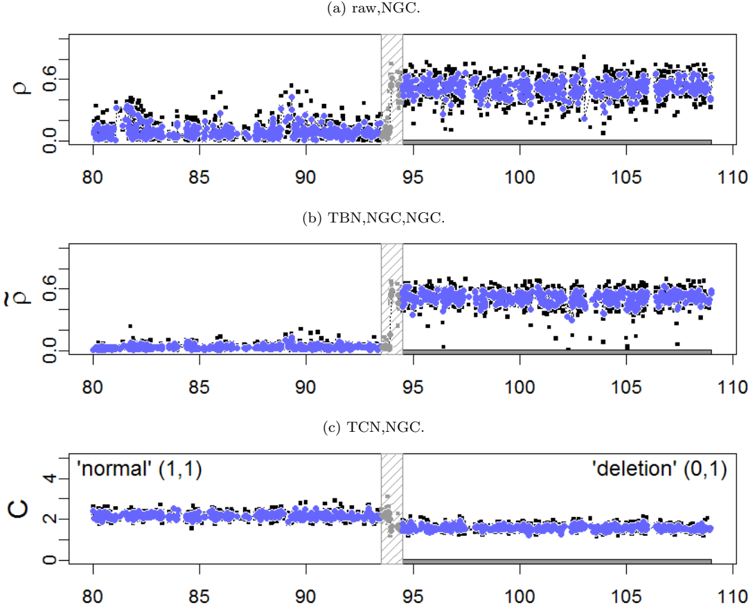
Figure 15: Decrease in Heterozygosity (DH) and total copy numbers for region TCGA-23-1027:Chr10@80-109,cp=94+/-0.5,s=0/2. Only heterozygous SNPs are plotted. There are 1582 loci of state 'normal' (1,1) ("negatives") and 1582 loci of state 'deletion' (0,1) ("positives"), where the latter are highlighted with a solid bar beneath. In total 98 loci within the safety margin were excluded.
