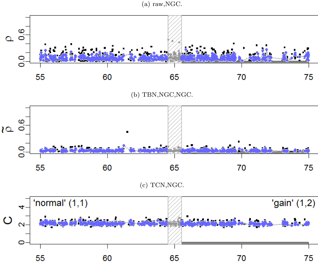
Figure 29: Decrease in Heterozygosity (DH) and total copy numbers for region TCGA-23-1027:Chr2@55-75.0,cp=65.0+/-0.5,s=0/1. Only heterozygous SNPs are plotted. There are 959 loci of state 'normal' (1,1) ("negatives") and 959 loci of state 'gain' (1,2) ("positives"), where the latter are highlighted with a solid bar beneath. In total 95 loci within the safety margin were excluded.
