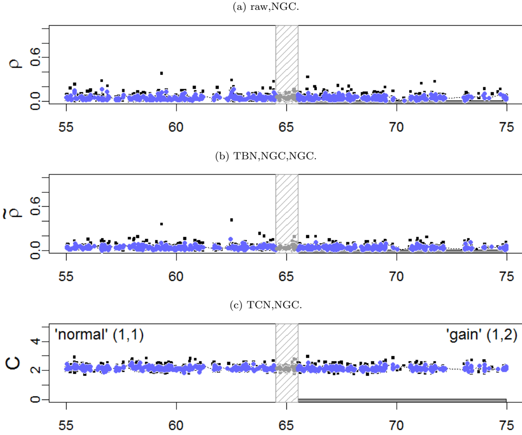
Figure 29: Decrease in Heterozygosity (DH) and total copy numbers for region TCGA-23-1027:Chr2@55-75.0,cp=65.0+/-0.5,s=0/1. Only heterozygous SNPs are plotted. There are 953 loci of state 'normal' (1,1) ("negatives") and 953 loci of state 'gain' (1,2) ("positives"), where the latter are highlighted with a solid bar beneath. In total 92 loci within the safety margin were excluded.
