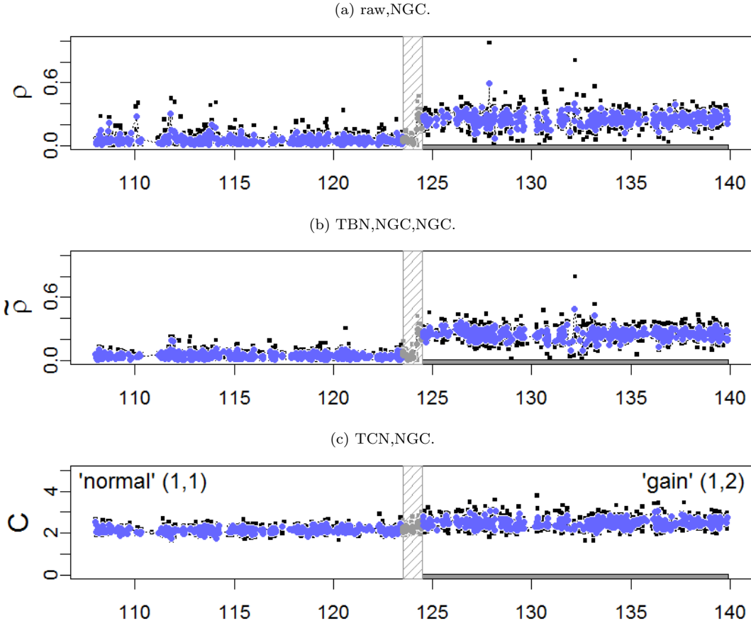
Figure 1: Decrease in Heterozygosity (DH) and total copy numbers for region TCGA-23-1027:Chr2@108-140,cp=124+/-0.5,s=0/1. Only heterozygous SNPs are plotted. There are 1620 loci of state 'normal' (1,1) ("negatives") and 1620 loci of state 'gain' (1,2) ("positives"), where the latter are highlighted with a solid bar beneath. In total 88 loci within the safety margin were excluded.
