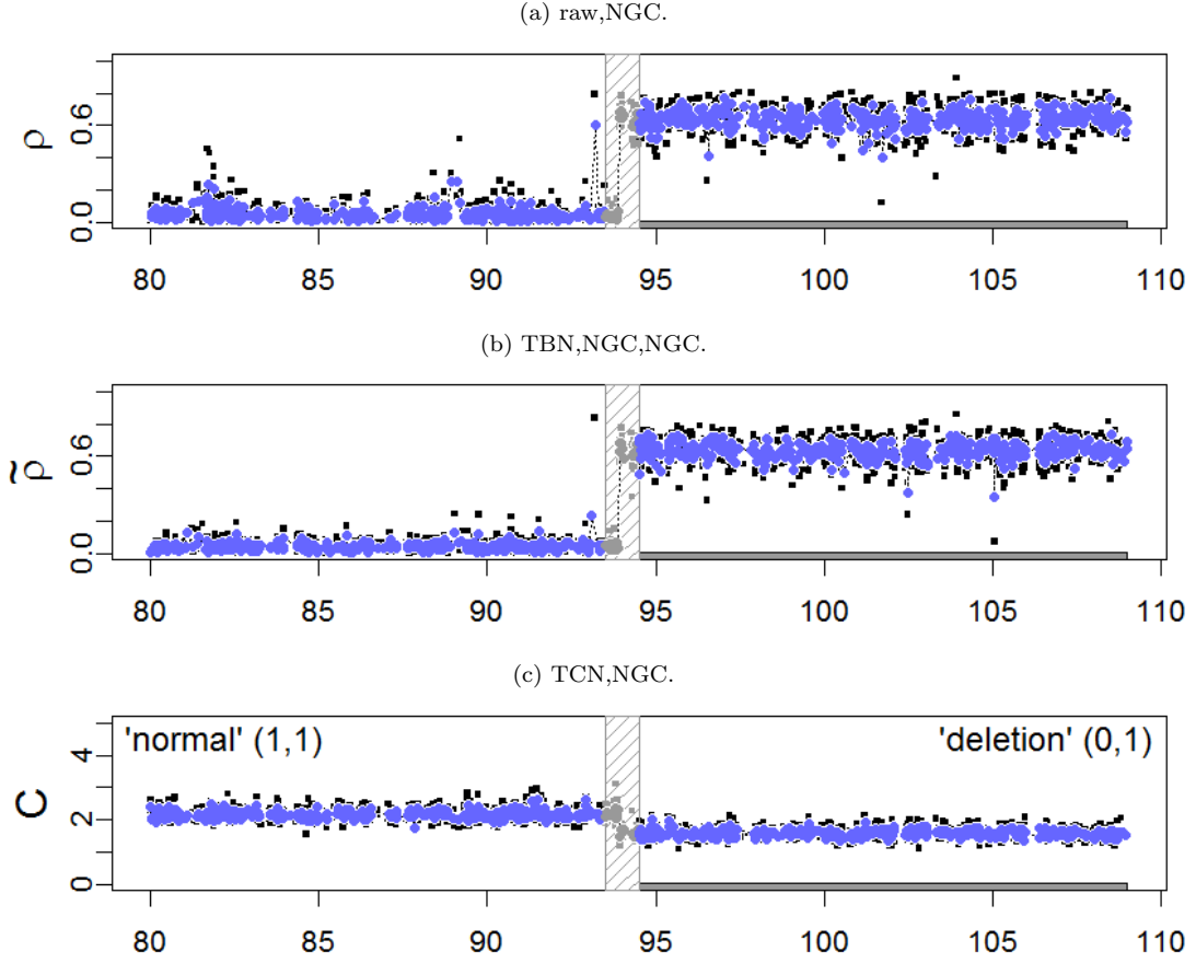
Figure 15: Decrease in Heterozygosity (DH) and total copy numbers for region TCGA-23-1027:Chr10@80-109,cp=94+/-0.5,s=0/2. Only heterozygous SNPs are plotted. There are 1568 loci of state 'normal' (1,1) ("negatives") and 1568 loci of state 'deletion' (0,1) ("positives"), where the latter are highlighted with a solid bar beneath. In total 97 loci within the safety margin were excluded.
