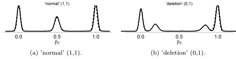
Figure 16: Density of raw (dashed lines) and TumorBoost-normalized (solid lines) allele B fractions for region TCGA-23-1027:Chr10@80-109,cp=94+/-0.5,s=0/2.
