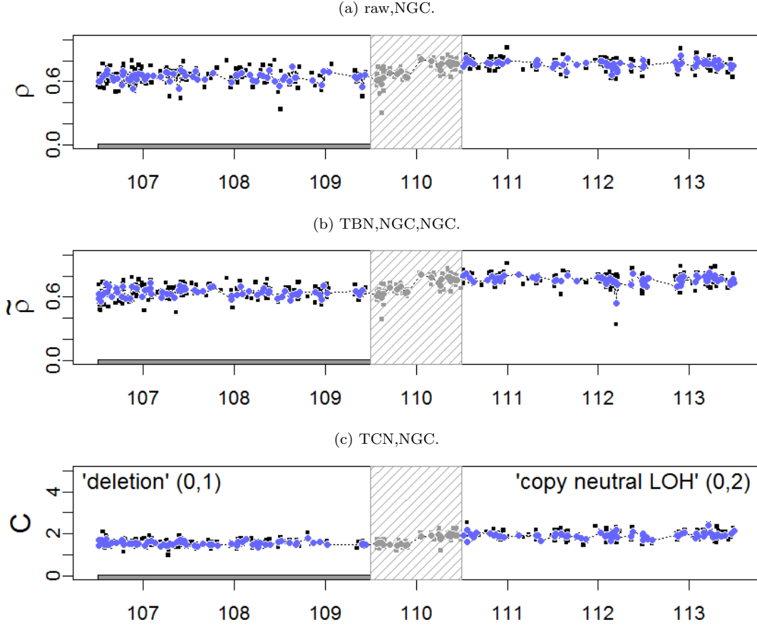
Figure 22: Decrease in Heterozygosity (DH) and total copy numbers for region TCGA-23-1027:Chr10@106.5-113.5,cp=110+/-0.5,s=2/3. Only heterozygous SNPs are plotted. There are 267 loci of state 'deletion' (0,1) ("negatives") and 267 loci of state 'copy neutral LOH' (0,2) ("positives"), where the latter are highlighted with a solid bar beneath. In total 80 loci within the safety margin were excluded.
