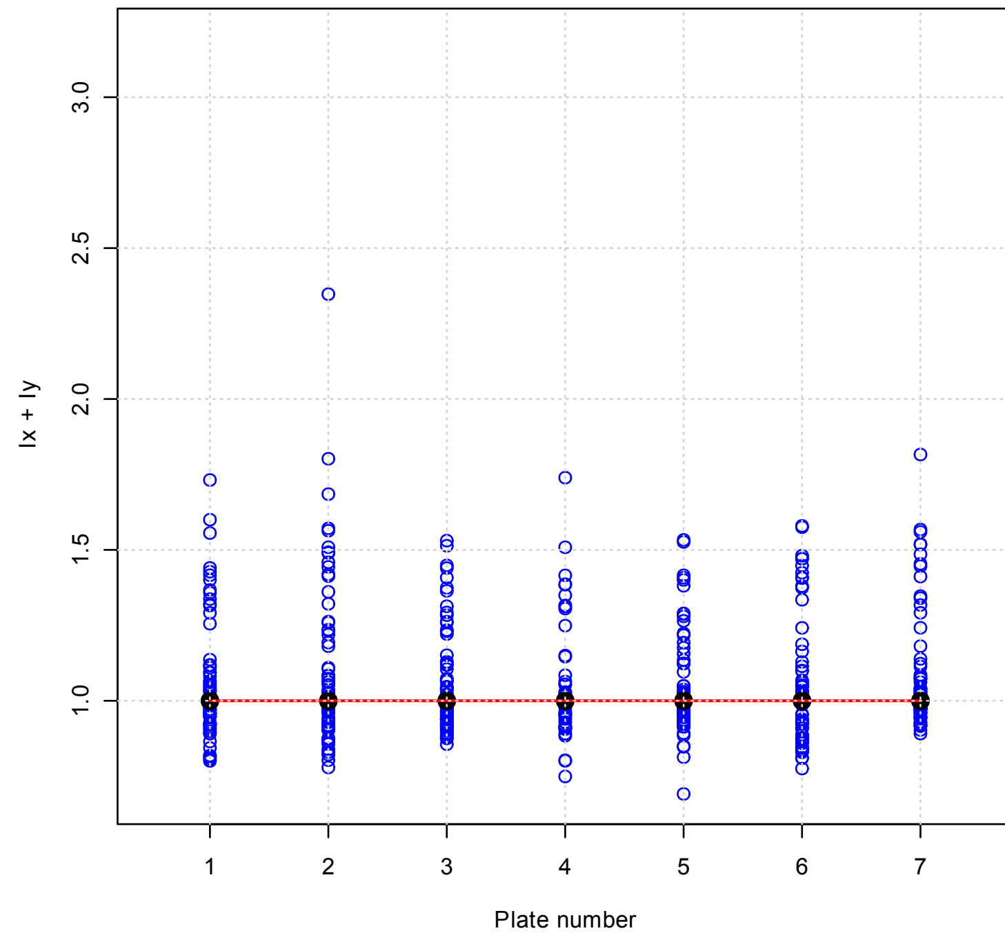
After per-plate-norm
