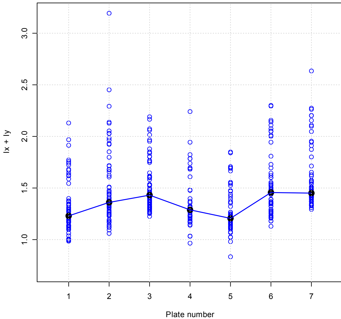
Before per-plate-norm
