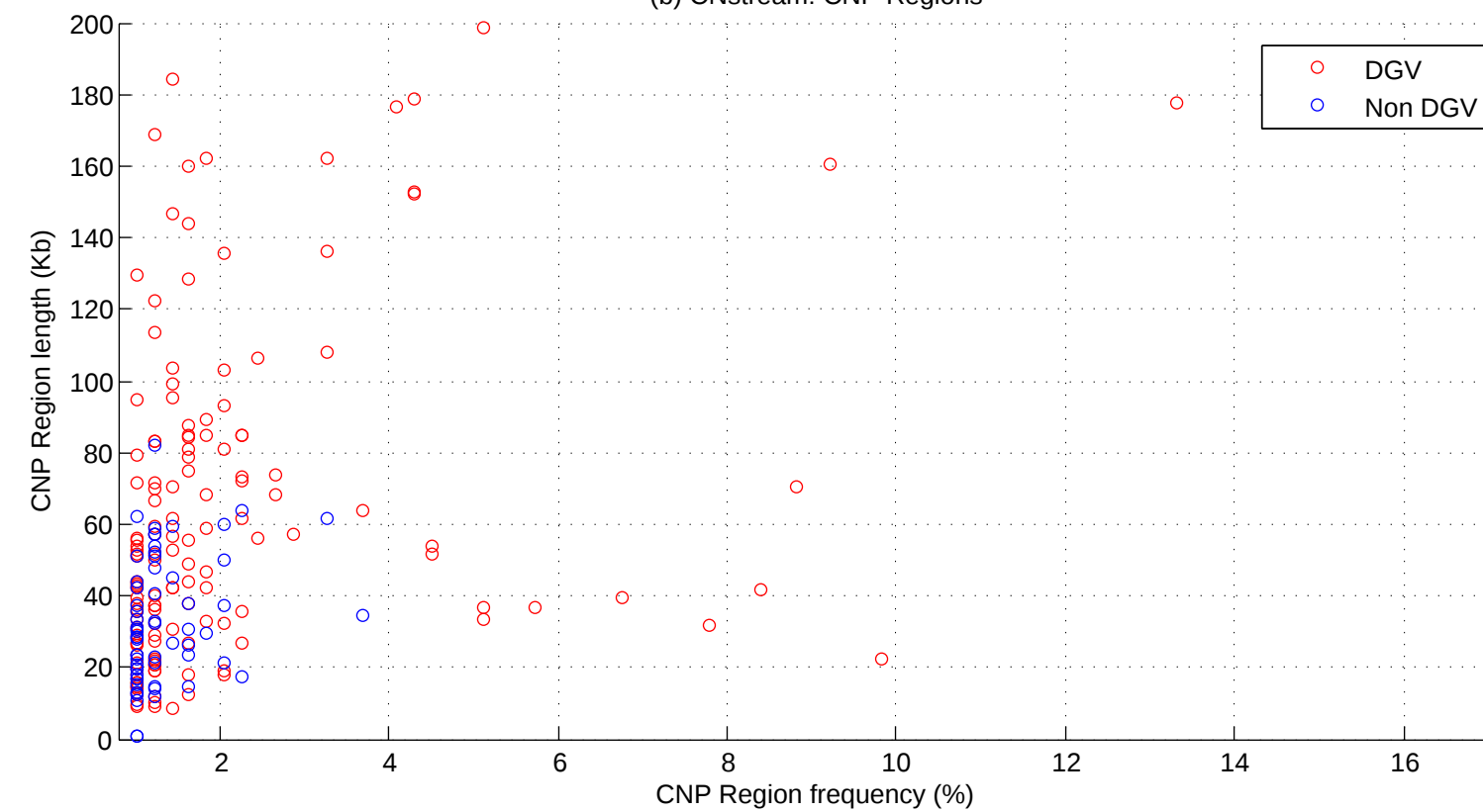
(b) CNstream: CNP Regions
