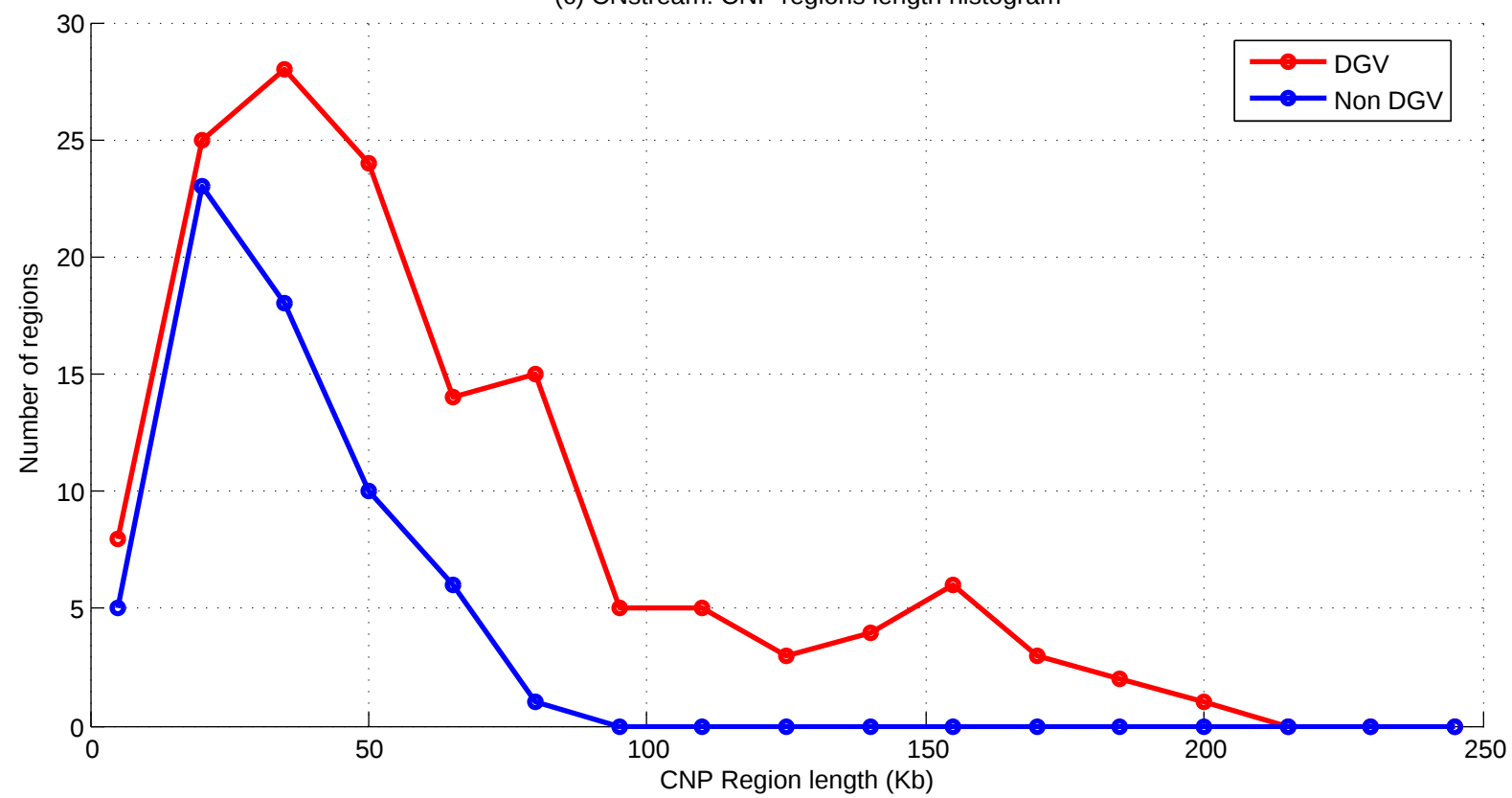
(c) CNstream: CNP regions length histogram
