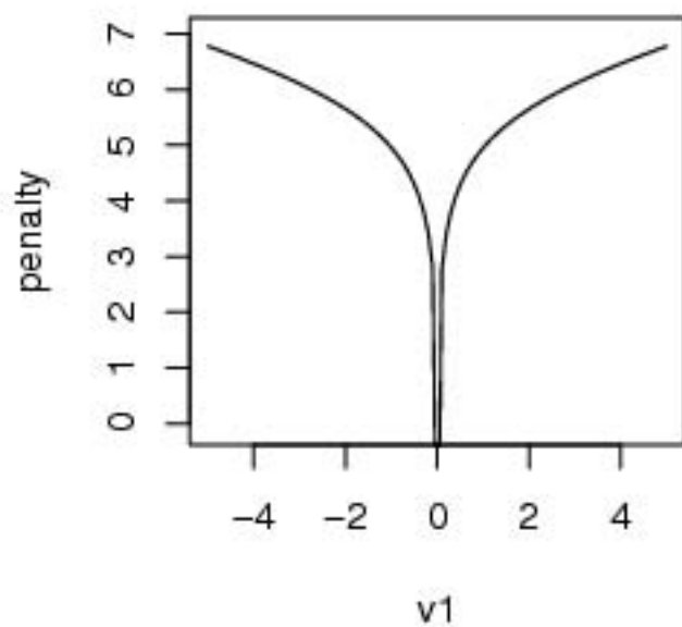
HL penalty with w=30
