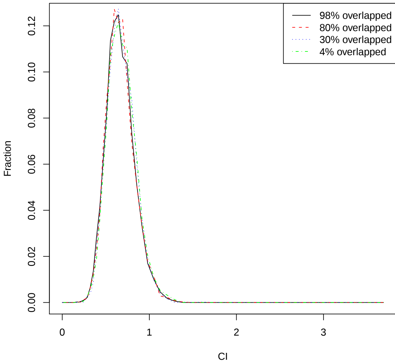
Distribution of CI against percentage overlapped
