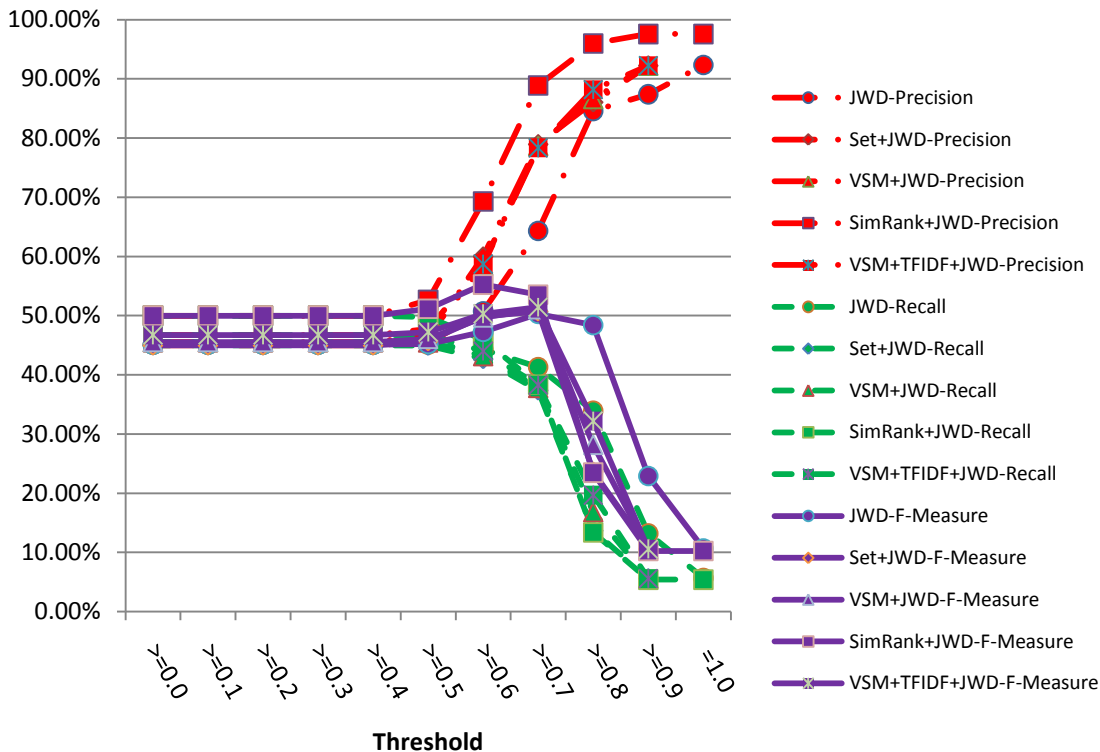
Precision, Recall and F-Measure
