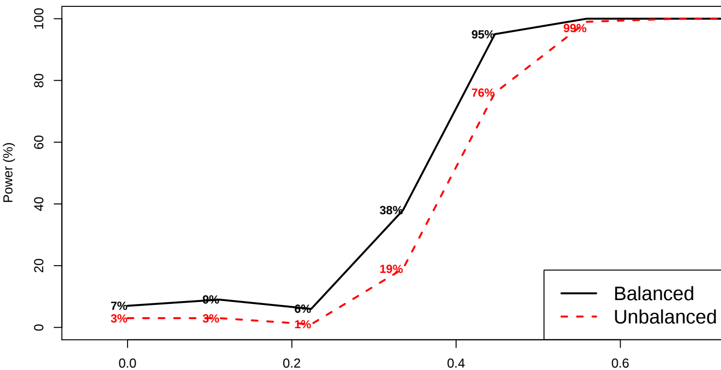
(a) KNN (n=150) 1% biomarkers
