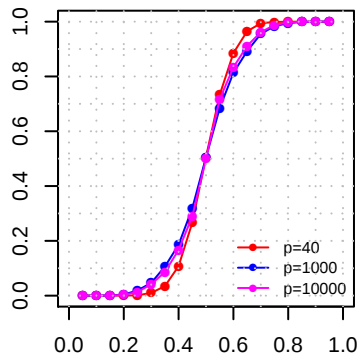
PAM
