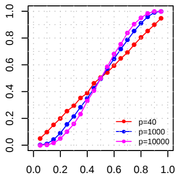
1-NN
