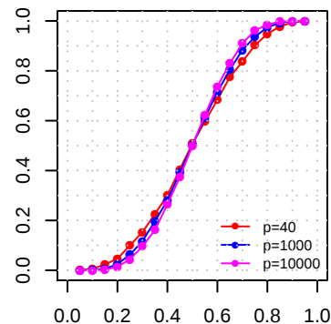
5-NN
