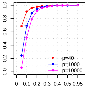
PAM
