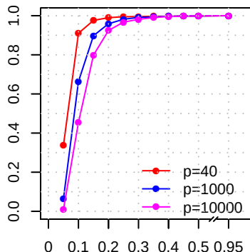
PAM
