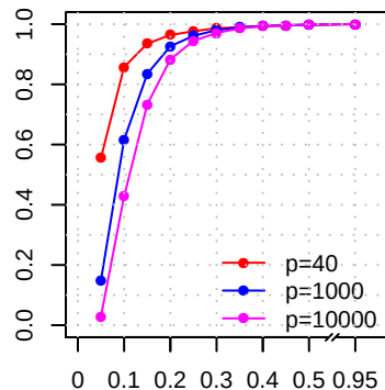
5-NN
