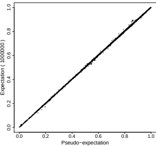
McCaskill model (Sensitivity)
