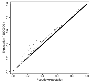
CONTRAFold model (PPV)
