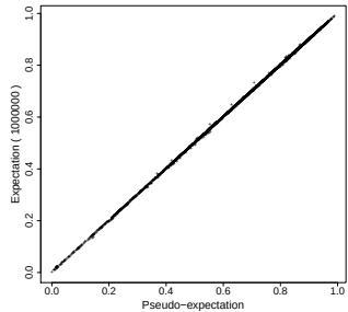
McCaskill model (F-score)
