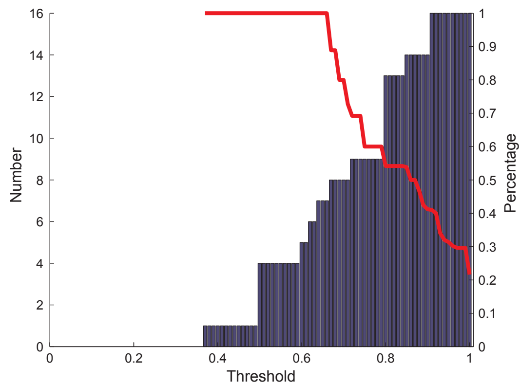
F-score
