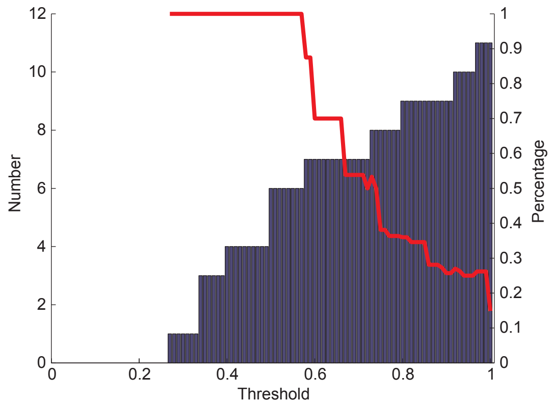
Sensitivity
