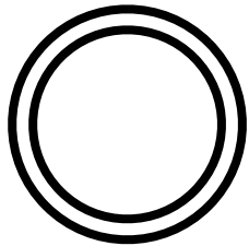
continuous place
