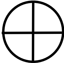
generic place
