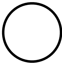
discrete place
