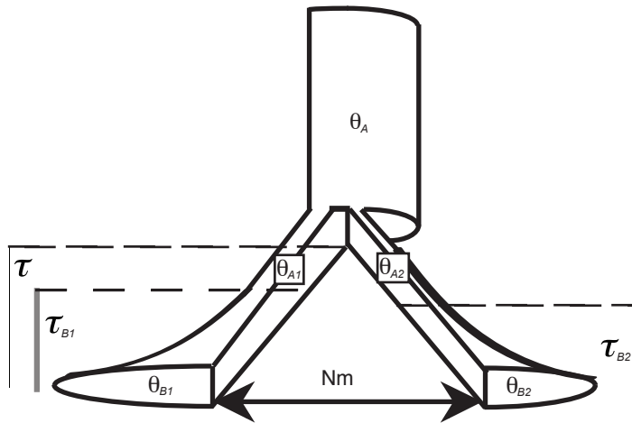
Migration Model
