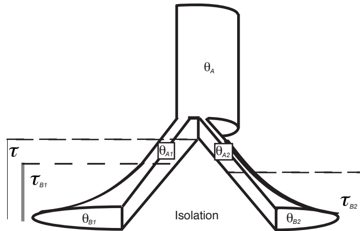
Isolation Model
