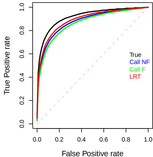
MAF=5% RR=1.5 at 5X
