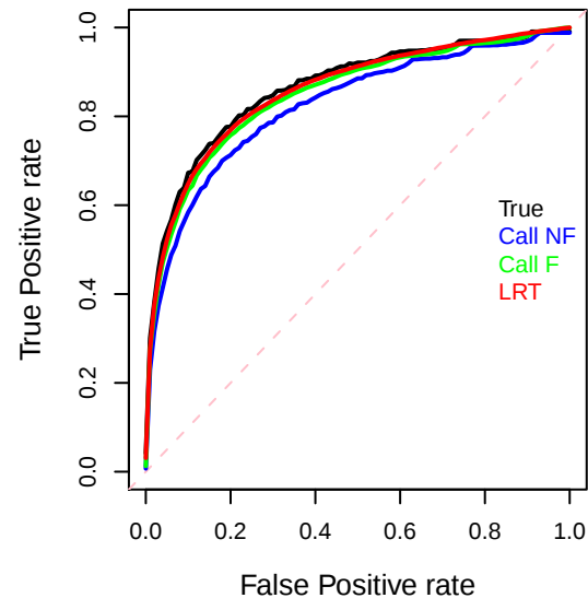
MAF=1% RR=2 at 10X
