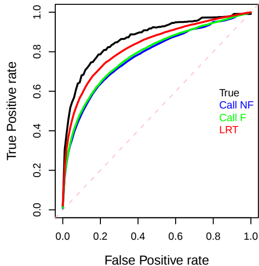
MAF=1% RR=2 at 5X
