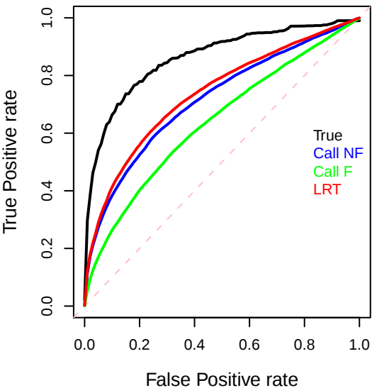
MAF=1% RR=2 at 2X
