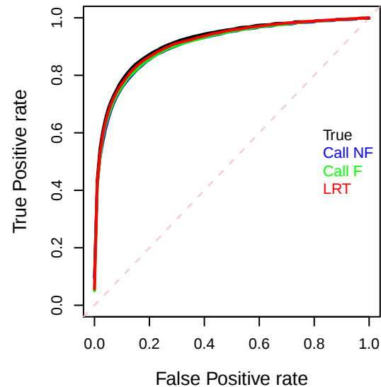
MAF=5% RR=1.5 at 10X
