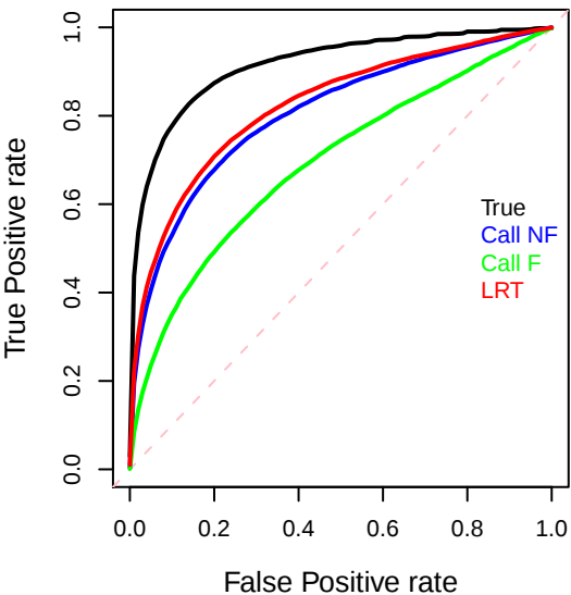
MAF=5% RR=1.5 at 2X
