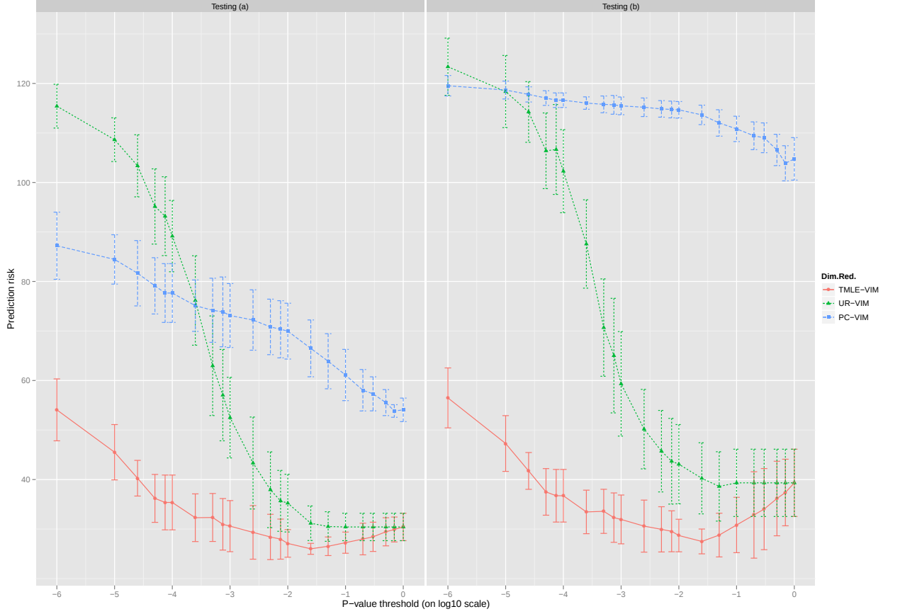
Figure 1: The prediction risk from the UR-VIM, the TMLE-VIM and the PCA for the simulation I data with setup (m_w = 10, \rho = 0.7, \sigma_e = 5) . D/S/A risks are plotted across a range of p-value thresholds that were used to truncate the variable (or component in the case of PCA) list in a dimension reduction procedure. The left panel plots prediction risks calculated on the testing set (a), and the right panel on the testing set (b). Red dots represent the TMLE-VIM, green triangles represent the UR-VIM, and blue squares represent the PCA. Standard error bars are superimposed on each point.
