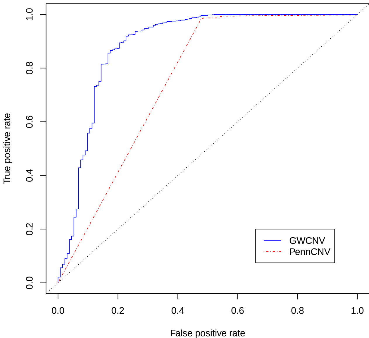
Chr16: Simulation ROC – CN 0 <RR = 1.8>
