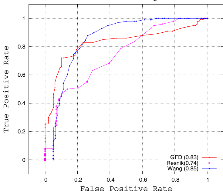
C) Cellular Component
