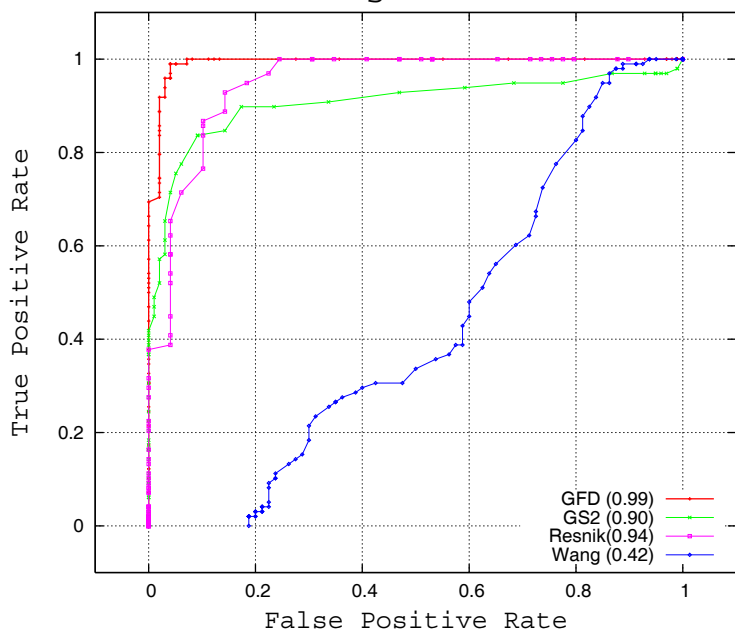
A) Biological Process
