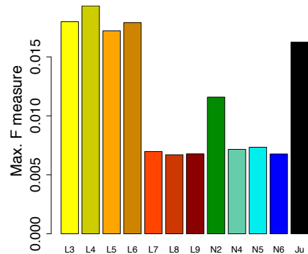
BINARY_PHYS – MirrorTree
