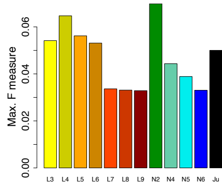
PATHWAYS – MirrorTree
