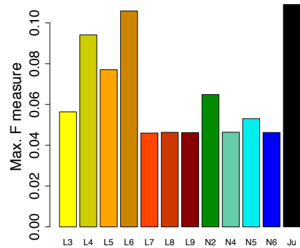
COMPLEXES – MirrorTree
