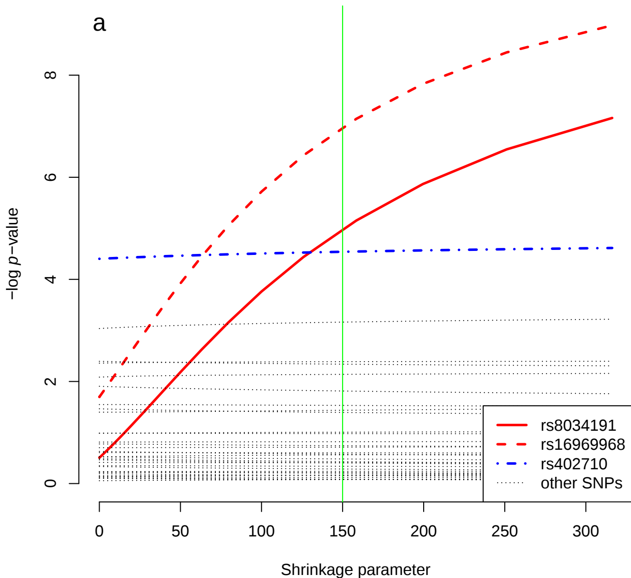
Approximate test
