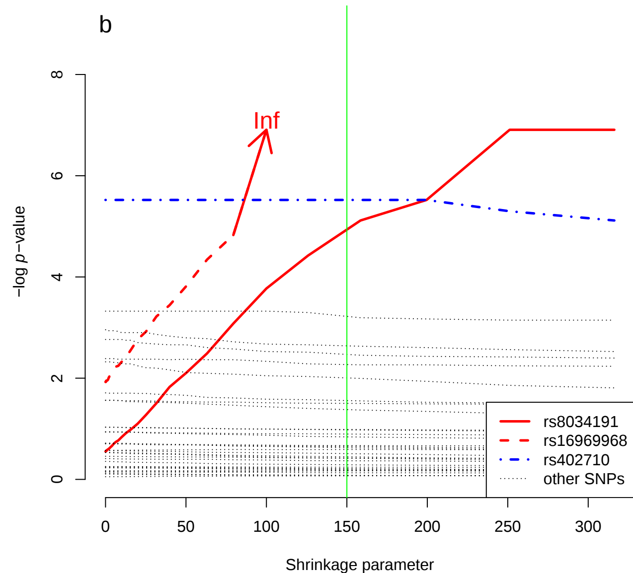
Permutation test
