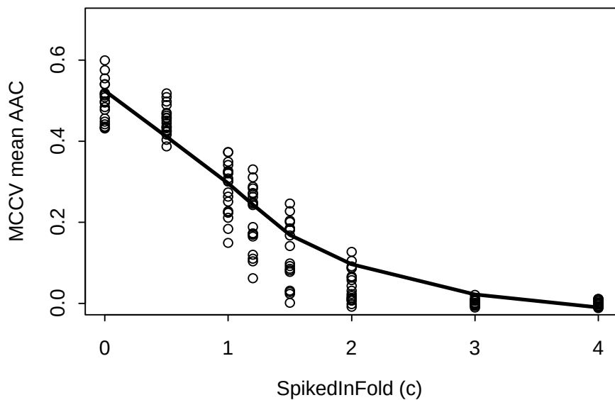
Gene:10, Feature:100, Sample:60
