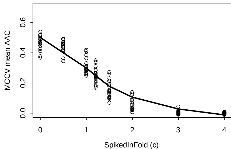
Gene:10, Feature:100, Sample:100
